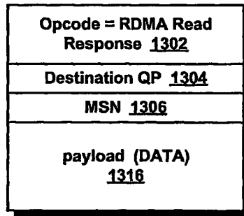
FIG. 13 (Related Art)
